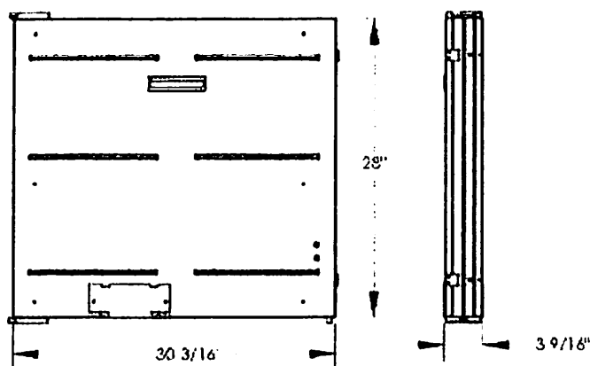
INSTALERT DIMENSIONS: FOLDED
