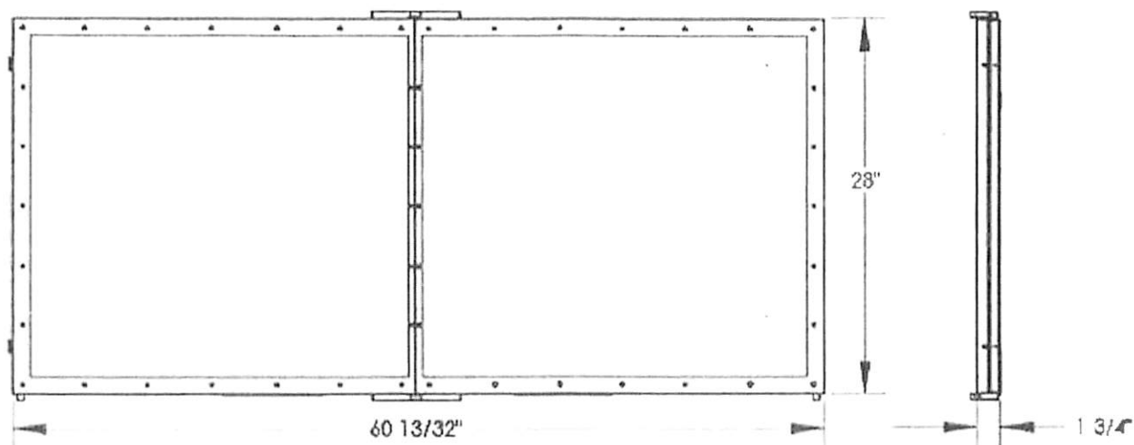
INSTALERT 24 DIMENSIONS: OPEN
