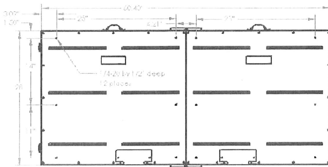
MOUNTING HOLE POSITIONS
